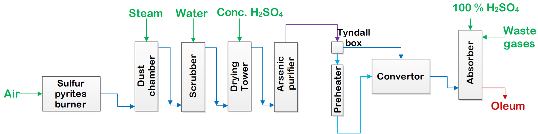
Figure: Manufacturing of Sulfuric acid by Contact process
